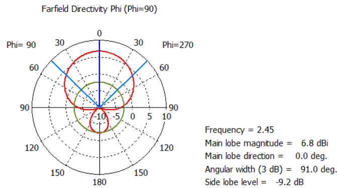
Fig 3 . Polar plot
