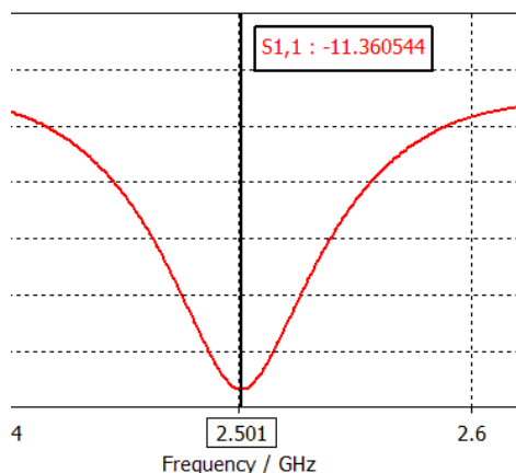
Fig 2. S11 of Aperture coupled antenna
