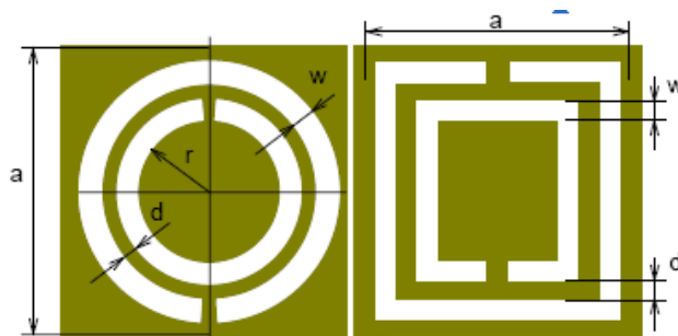
Fig 4. CSRR unit cell structure
