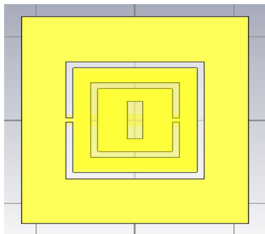
Fig 6. Metamaterial Microstrip patch antenna
