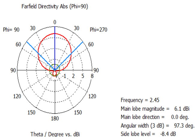
Fig 8 . Graph of Polar plot
