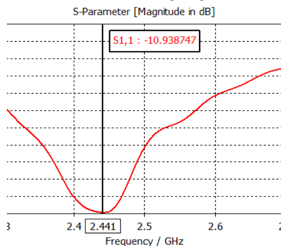
Fig 7 . Graph of S11 using Metamaterial
