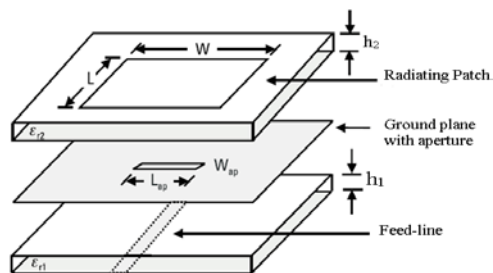
Fig 1. Aperture coupled microstrip antenna
