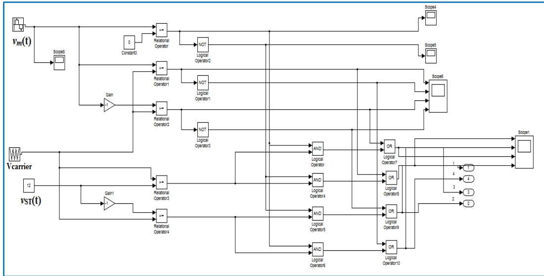
Fig. 5 Simulink model of PWM generation circuit.
