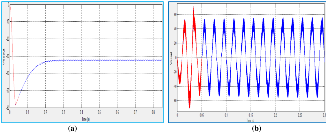
Fig.9 (a) DC output voltage waveform, (b) AC output voltage waveform
