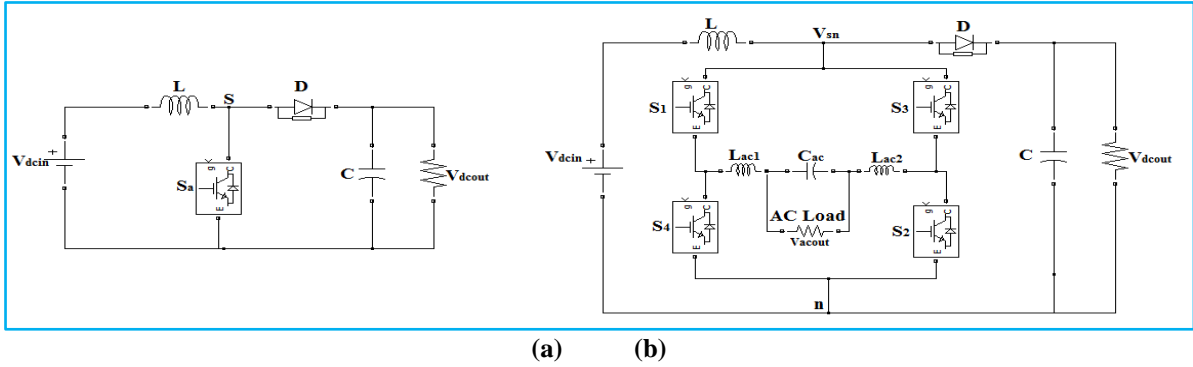
Fig 2. (a) Conventional boost converter, (b) Proposed Boost-Derived Hybrid converter obtained by replacing S_a with a single phase bridge network.
