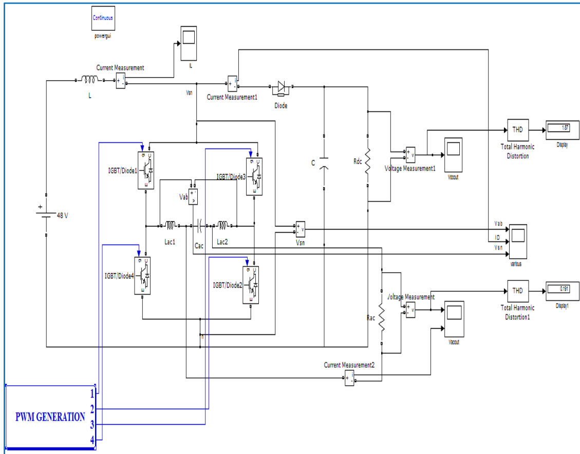
Fig. 4 Simulink model of Boost derived Hybrid converter.
