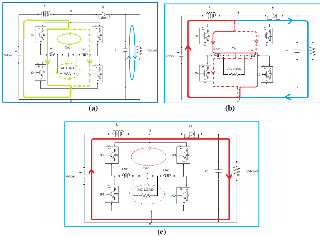
Fig. 3(a) Shoot-Through interval, (b) Power interval and (c) Zero interval.
