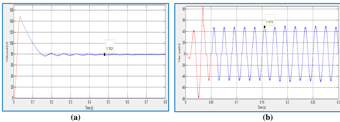
Fig.7 (a) Output DC voltage waveform, (b) Output AC voltage waveform.
