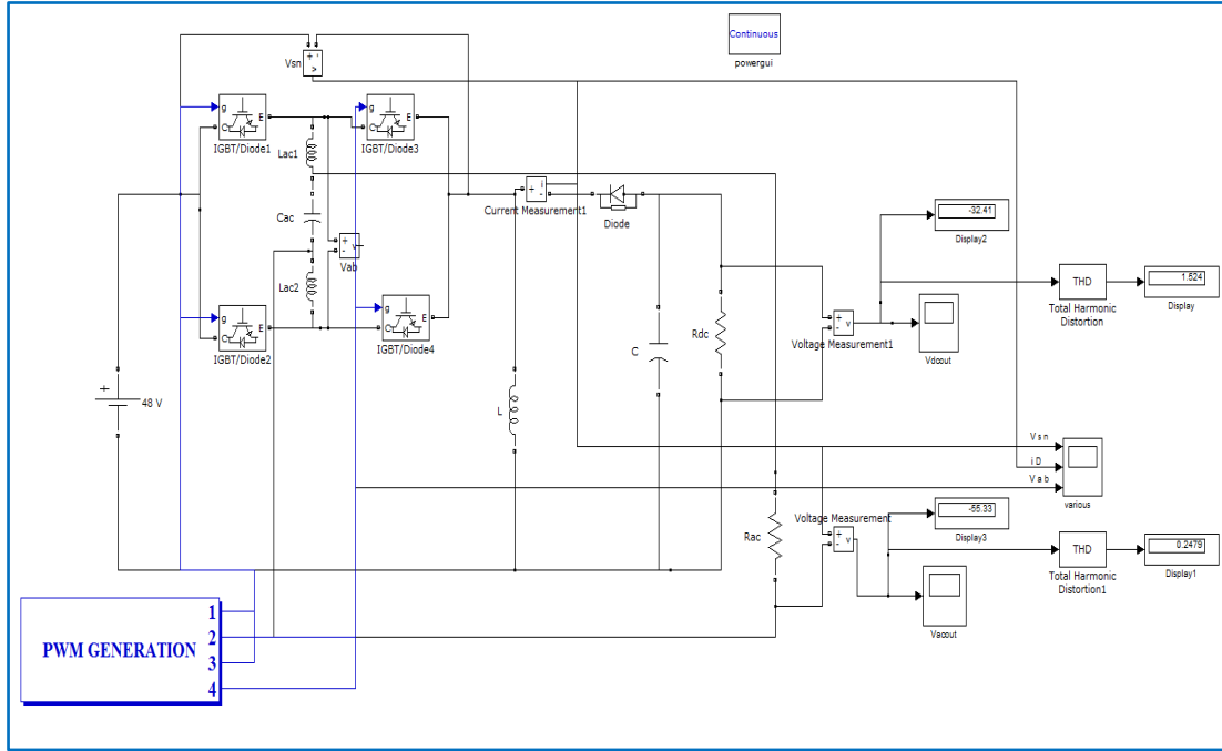
Fig.8 Simulink model of Buck-Boost derived hybrid converter.
