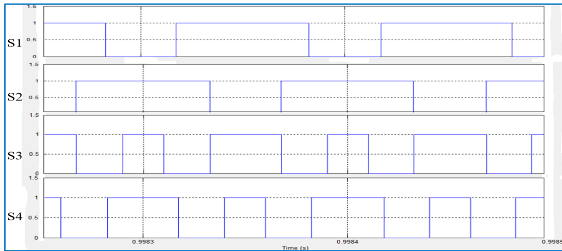
Fig. 6 Control signals to the switches S_1 - S_4 .
