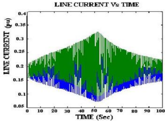
Fig.7 (d) System Response for 2-Machine System with TCSC without damping Controller-Line Currents
