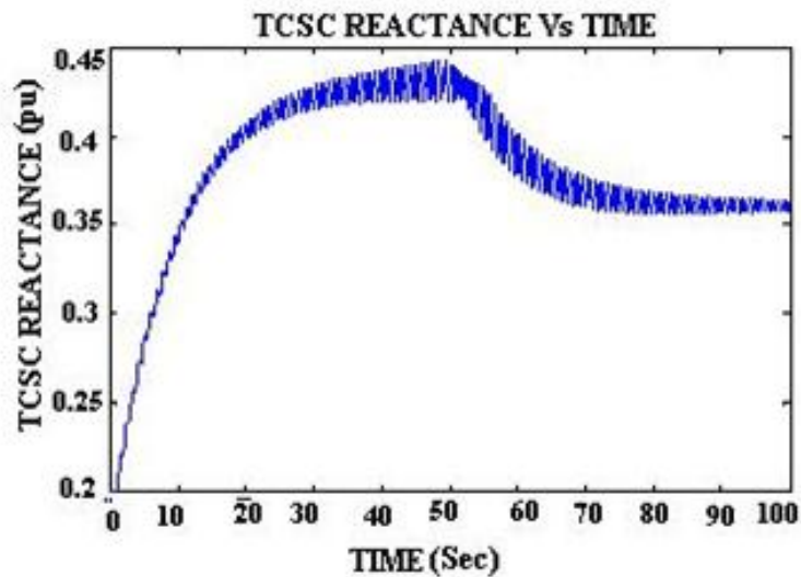
Fig.7(a) System Response for 2-Machine System with TCSC without damping Controller-TCSC reactance
