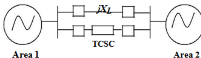
Fig. 1 Two Machine System with TCSC Controller
