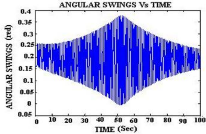
Fig.7(c) System Response for 2-Machine System with TCSC without damping Controller - Angular Swings
