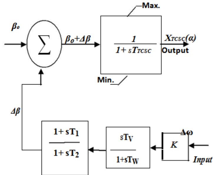
Fig. 4 Structure of TCSC Controller
