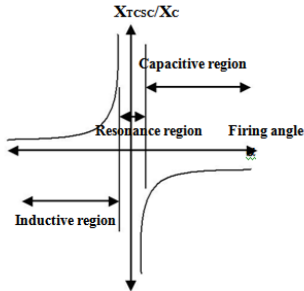
Fig. 3 X_{Tcsc} / X_c Vs FIRING ANGLE ( \alpha ) CURVE
