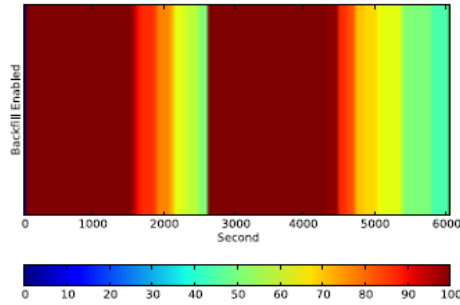
Figure 6. IaaS cloud infrastructure utilization with on-demand user VMs and backfill VMs processing Condor jobs.
