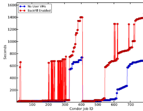
Figure 8. Condor job queued time when the job begins executing for the last time before successful completion, using the most recent backfill termination policy.
