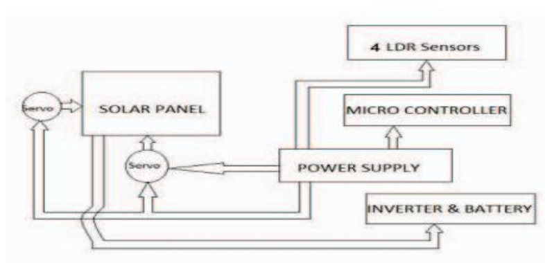
Fig. 4. Block diagram of overall system
