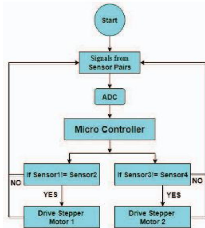
Fig. 5. Control algorithm
