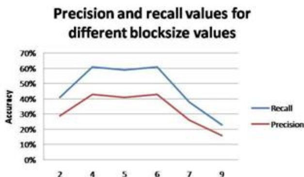
Fig. 13. Effect of block size change using HOG method. The number of bins is constant 9.
