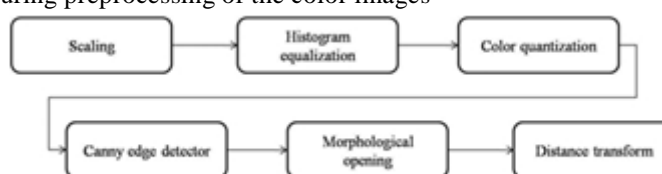
Fig. 4. The steps of preprocessing.
