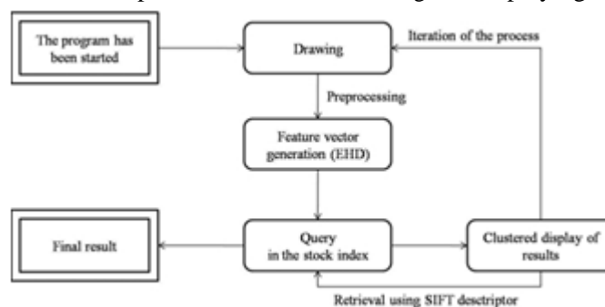
Fig. 2. The data flow model of the system from the user's point of view. subsystem (GUI). The global
