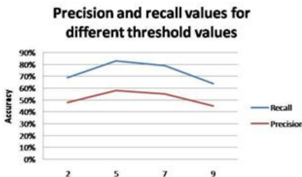
Fig. 12. Effect of threshold value change using EHD method. The block size is constant 10.
