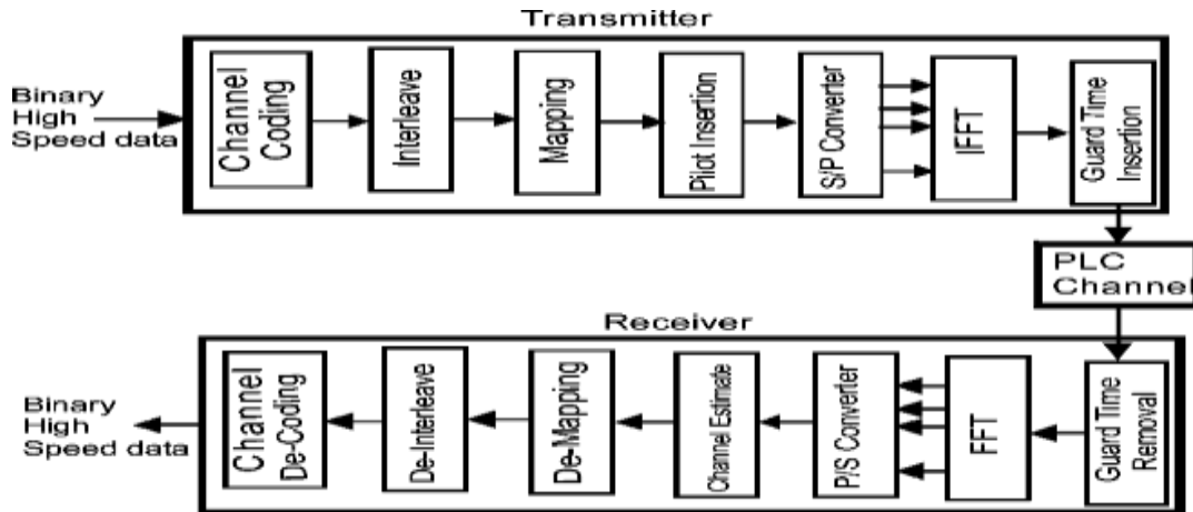
Fig: 2 - power line channel block diagram of transmitter and receiver
