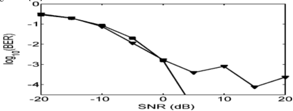
Fig:4. PLC Performance in a noise limited channel
