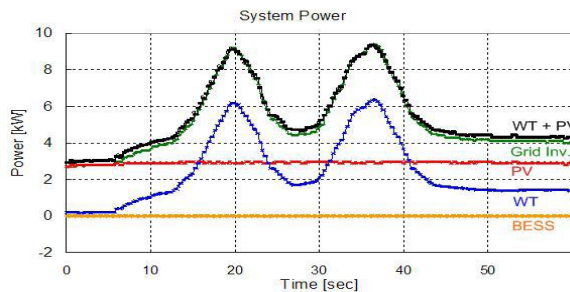
Fig. 5. Experimental results for normal operation mode
