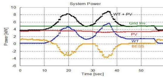
Fig. 6. Experimental results for power dispatching mode
