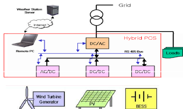
Fig. 1. A configuration of the proposed hybrid generation system
