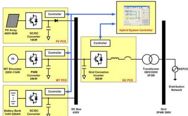
Fig. 2. A block diagram of the proposed hybrid generation system
