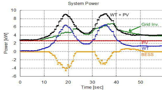
Fig. 7. Experimental results for power averaging mode
