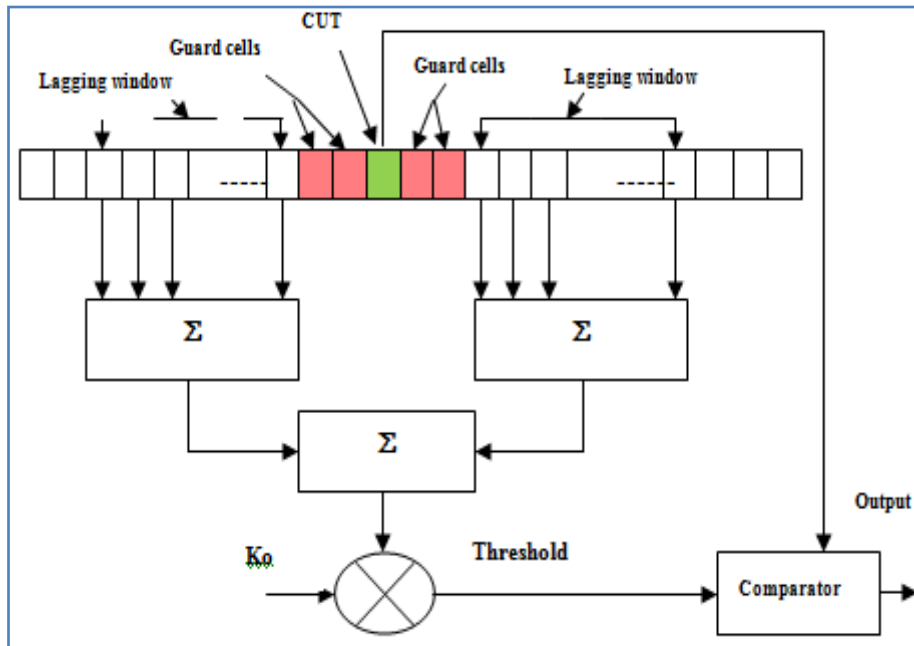
Fig.2 Cell Averaging CFAR (CA-CFAR).
