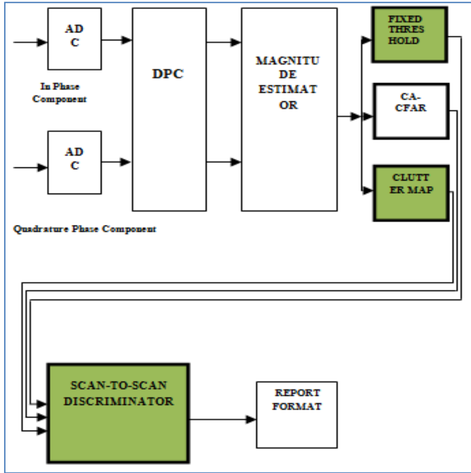
Fig.3 Functional block diagram.
