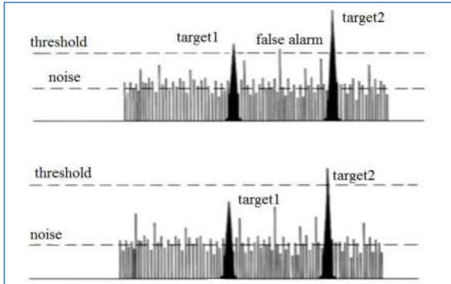
Fig.1 Detection of target using fixed threshold.
