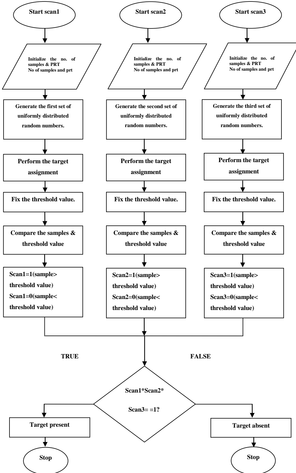
Fig.4 Flow chart for scan-to-scan discriminator using fixed threshold.
