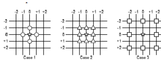
Figure 4: Refinement vectors in three different cases
