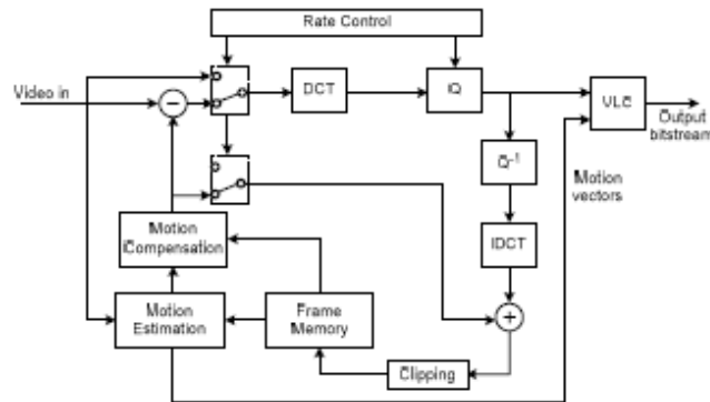
Fig 2: The structure of the proposed Encoder
