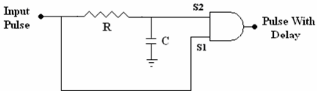
Fig: 4(a) Dead Time Generator.
