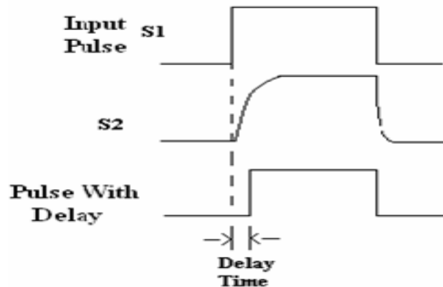
Fig: 4(b) Waveforms Of Dead Time Generator.
