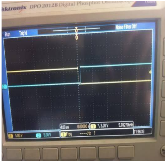
Fig: 4(e) Rising Edge ( Dead Band Created)
