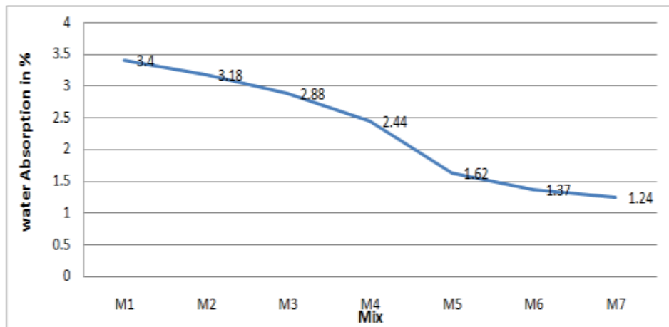
Figure7 Water Absorption for various mixes
