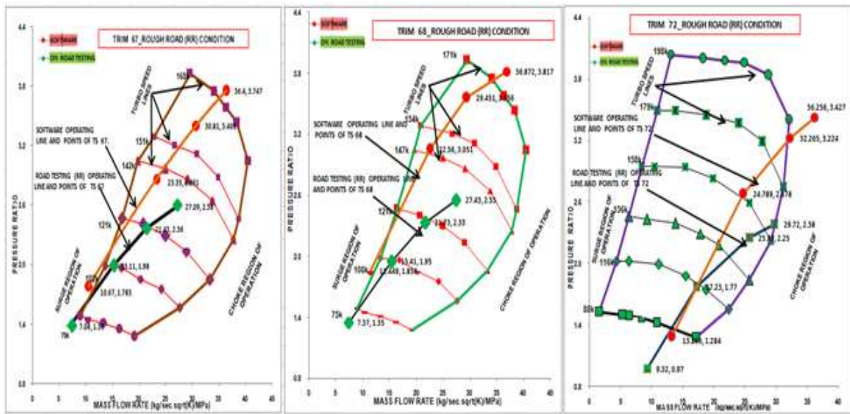
Fig. 2 B60J67, B60J68 and A58N72 Turbo-match- by Simulation & Data-logger – Rough Road
