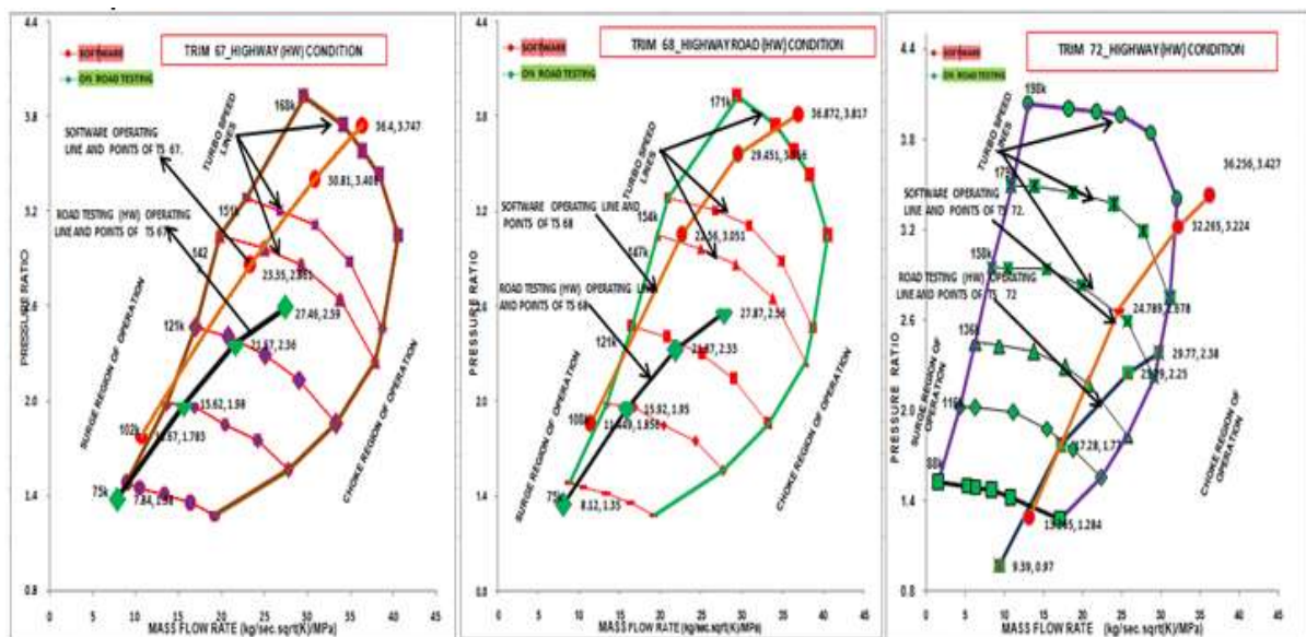
Fig. 3 B60J67, B60J68 and A58N72 Turbo-match- by Simulation & Data-logger – Highway Route
