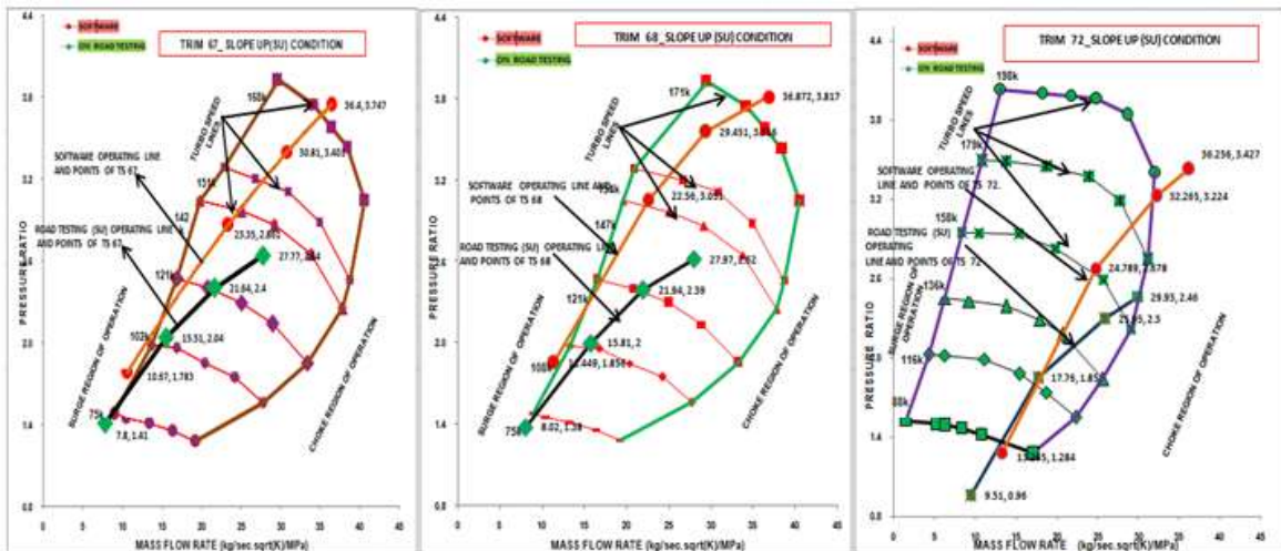
Fig. 5 B60J67, B60J68 and A58N72 Turbo-match- by Simulation & Data-logger – Slope-up Route
