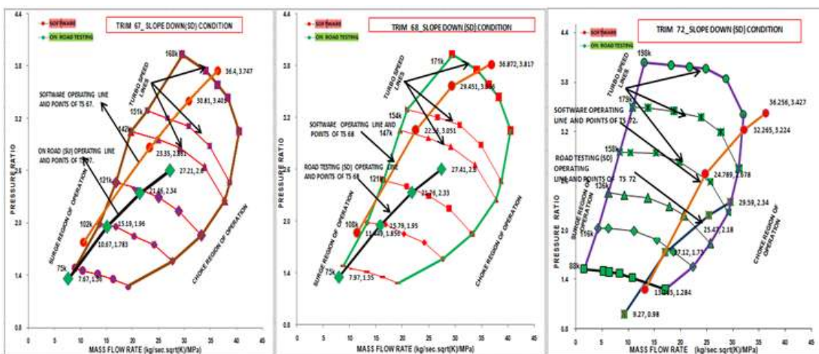
Fig. 6 B60J67, B60J68 and A58N72 Turbo-match- by Simulation & Data-logger – Slope-Down Route
