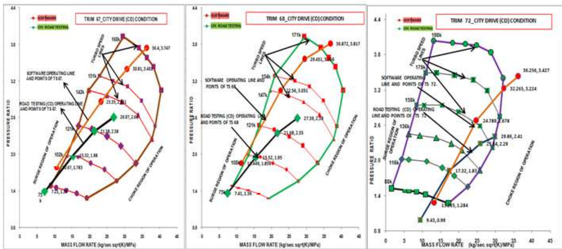
Fig. 4 B60J67, B60J68 and A58N72 Turbo-match- by Simulation & Data-logger – City Route
