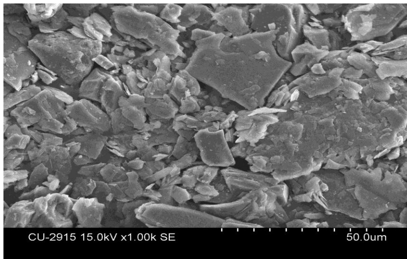
Figure 8a. SEM observation of the surface of \text{CaCO}_3 and NR/ \text{CaCO}_3 composite for unmodified \text{CaCO}_3 (1000X)
