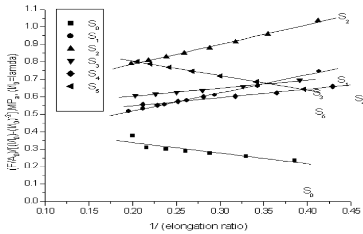
Figure 5b. Mooney – Rivlin plot of \text{CaCO}_3 filled NR vulcanizates samples at moderate elongations
