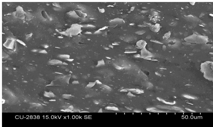
Figure 8e SEM observation of the surface of \text{CaCO}_3 and NR/ \text{CaCO}_3 composite for 40 phr \text{CaCO}_3 /NR composite ( S_2 ) (1000X)
