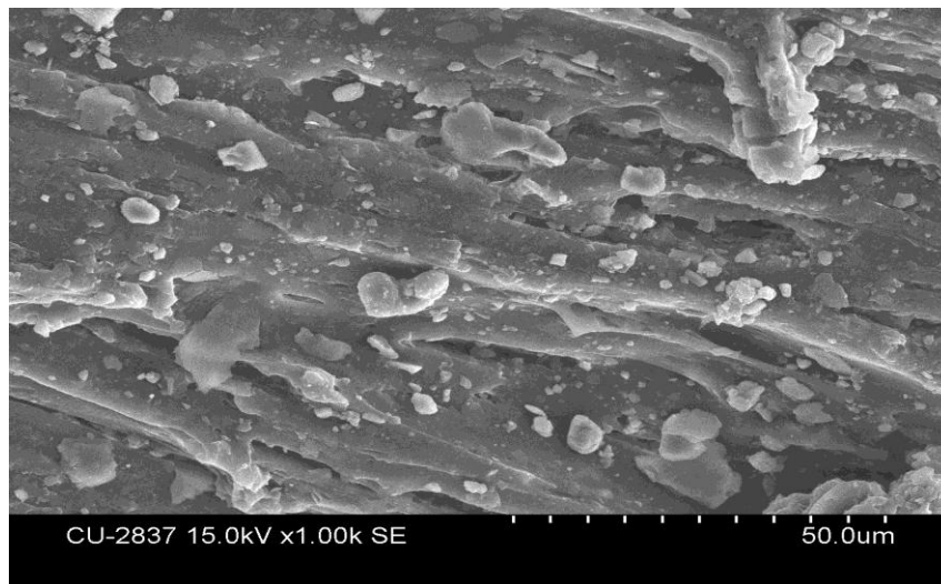
Figure 8d. SEM observation of the surface of \text{CaCO}_3 and NR/ \text{CaCO}_3 composite for 20 phr \text{CaCO}_3 /NR composite ( S_1 ) (1000X)
