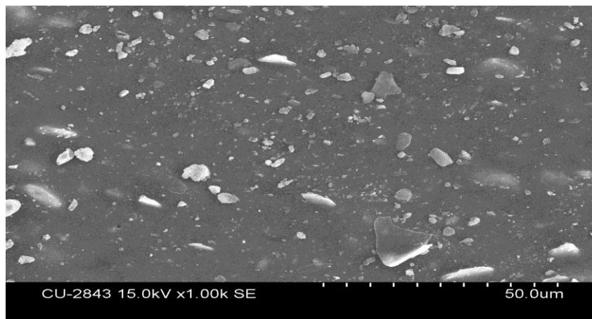
Figure 8g. SEM observation of the surface of \text{CaCO}_3 and NR/ \text{CaCO}_3 composite for 15 phr modified \text{CaCO}_3 /NR composite ( S_4 ) (1000X)
