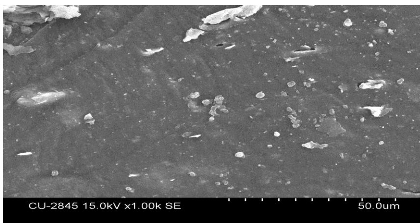
Figure 8h. SEM observation of the surface of \text{CaCO}_3 and NR/ \text{CaCO}_3 composite for 20 phr modified \text{CaCO}_3 /NR composite ( S_5 ) (1000X)
