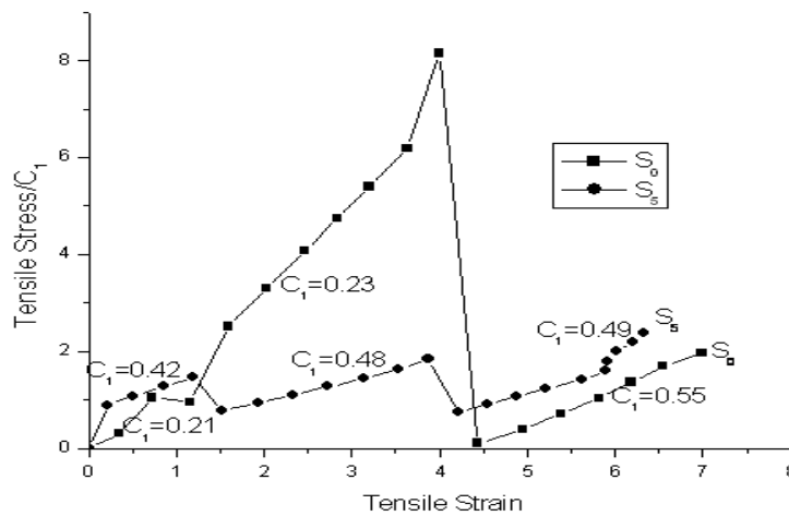
Figure 6. \sigma/C_1 versus \epsilon plot for S0 vulcanizate at various strain having different C_1 values
