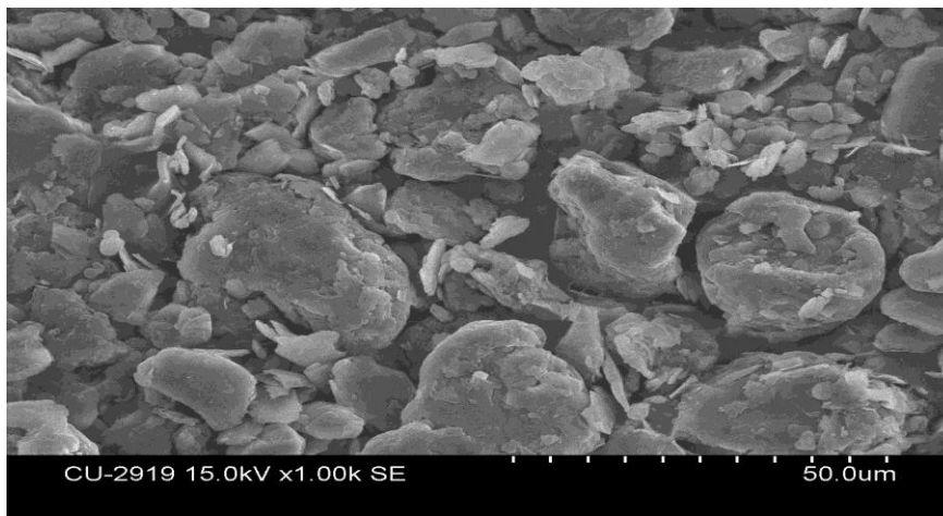
Figure 8b. SEM observation of the surface of \text{CaCO}_3 and NR/ \text{CaCO}_3 composite for PMMA modified \text{CaCO}_3 (1000X)
