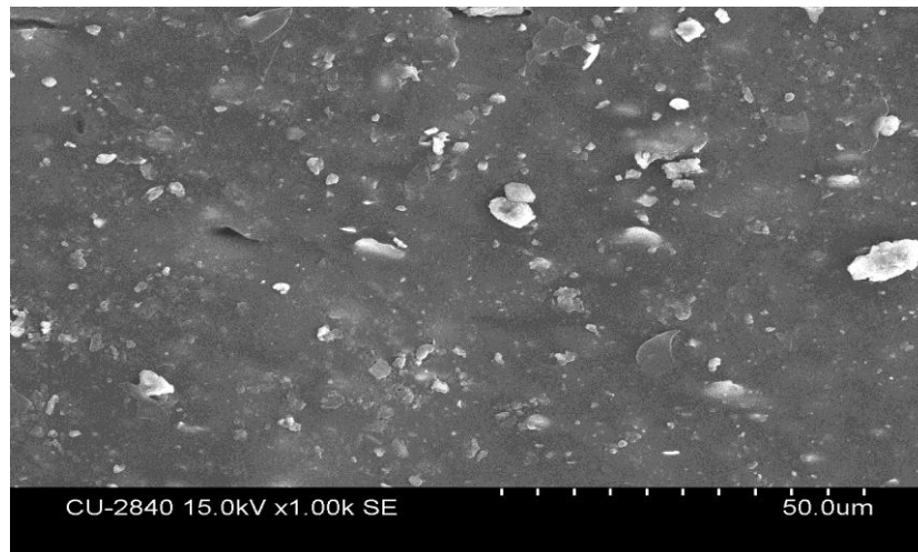
Figure 8f. SEM observation of the surface of \text{CaCO}_3 and NR/ \text{CaCO}_3 composite for 10 phr modified \text{CaCO}_3 /NR composite ( S_3 ) (1000X)
