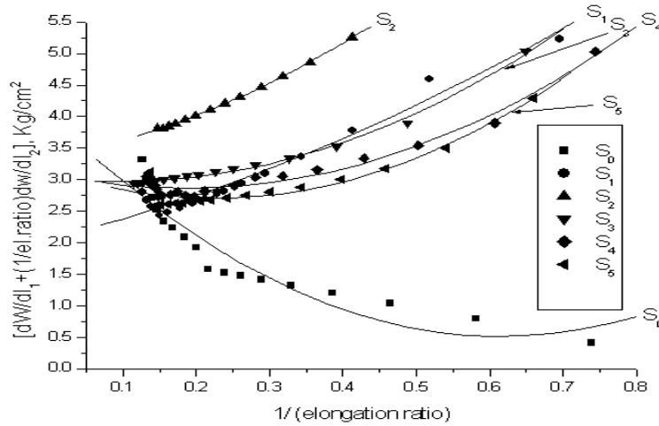
Figure 7. Plots of \left[ \frac{\partial W}{\partial \lambda_1} + \frac{\partial W}{\partial \lambda_2} \lambda^{-1} \right] vs 1/\lambda for \text{CaCO}_3 -NR composite vulcanizates on simple extension.
