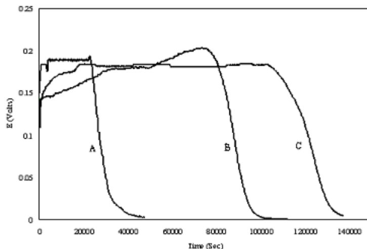
Fig. 4. Voltage transients monitored during electro-oxidation using 10 vol. % methanol solution for DMFC with Ni-coated anode polar plate: (A) 1.1 cm 3 , (B) 3.3 cm 3 and (C) 4.4 cm 3 .
