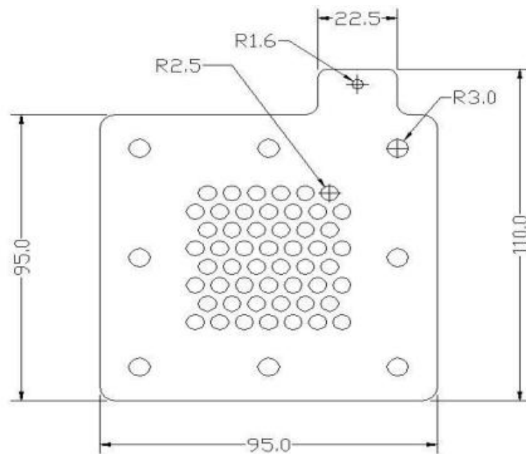
Fig. 2. Dimensions of bipolar plate.
