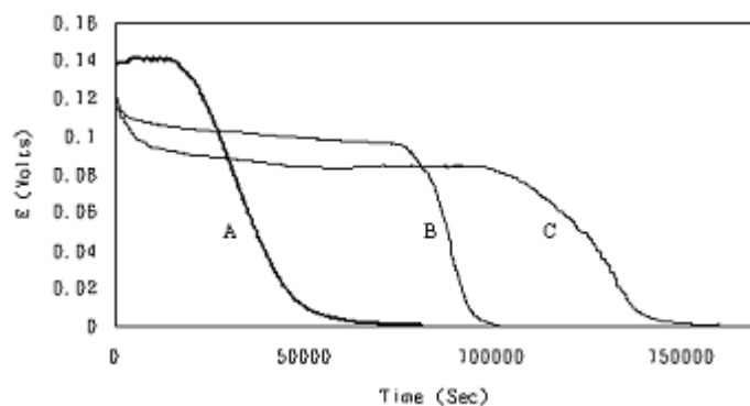
Fig. 6. Voltage transients monitored during electro-oxidation using 10 vol. % methanol solution for DMFC with uncoated anode polar plate: (A) 1.1 cm 3 , (B) 3.3 cm 3 and (C) 4.4 cm 3 .
