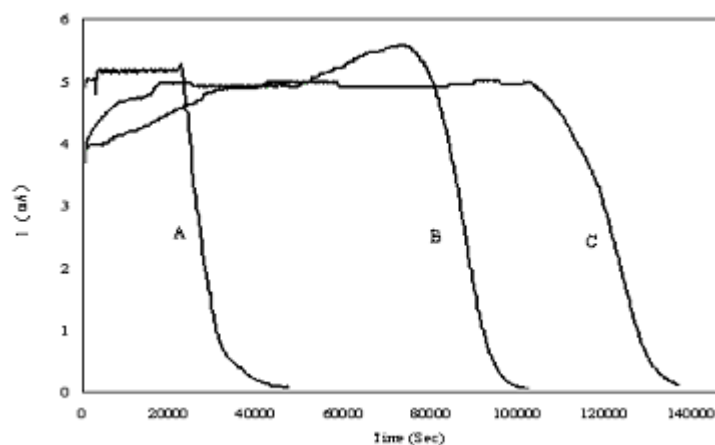
Fig. 5. Current transients monitored during electro-oxidation using 10 vol. % methanol solution for DMFC with Ni-coated anode polar plate: (A) 1.1 cm 3 , (B) 3.3 cm 3 , and (C) 4.4 cm 3 .
