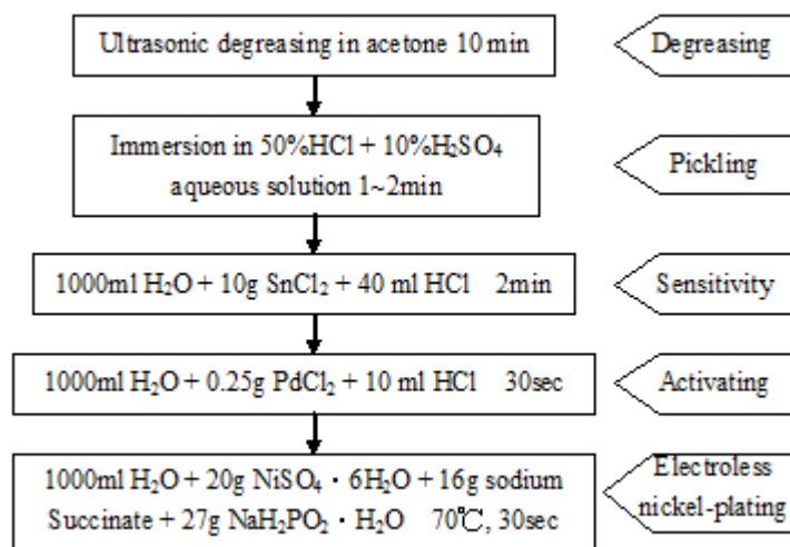
Fig. 3. Flow chart of preparing the nickel - plating by an electroless method.
