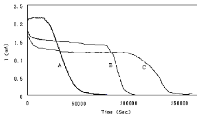
Fig. 7. Current transients monitored during electro-oxidation using 10 vol. % methanol solution for DMFC with uncoated anode polar plate: (A) 1.1 cm 2 , (B) 3.3 cm 2 and (C) 4.4 cm 2 .
