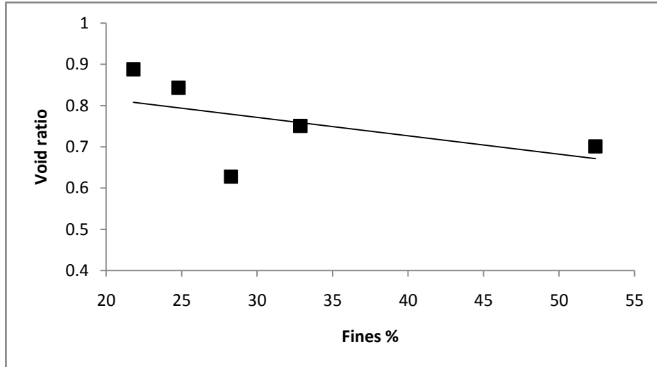
Fig.7 Variation of Void ratio with Fines (%)
