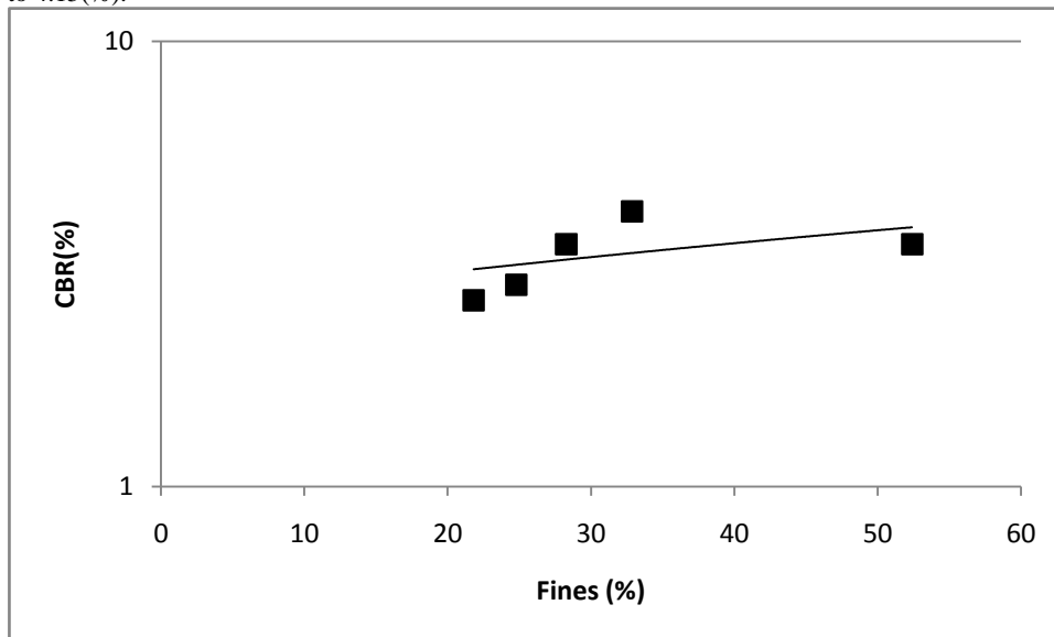
Fig.8 Variation of CBR with Fines (%)
