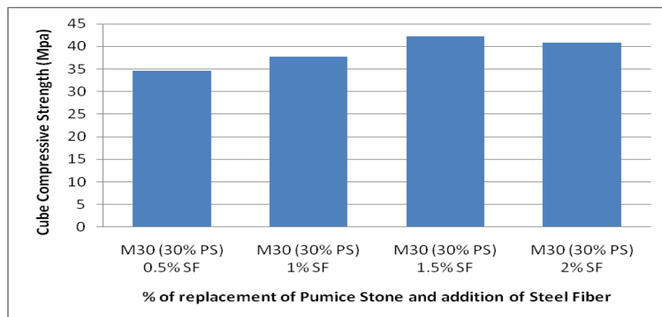
Fig. 3 Cube Compressive Strength (Mpa) with the replacement of Pumice Stone & addition of Steel Fiber
