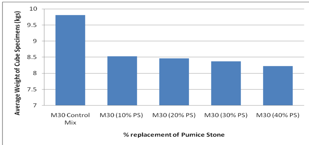
Fig.2 Average Weight of Cube Specimens (kgs)
