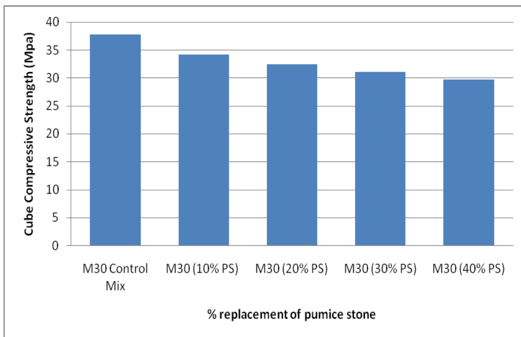
Fig: 1 Cube Compressive Strength (Mpa) with the replacement of Pumice Stone
